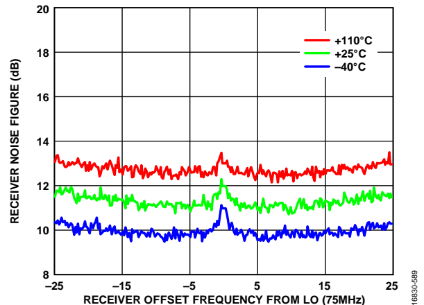
Figure 11. Receiver Noise Figure vs. Receiver Offset Frequency from LO, Integration Bandwidth = 200 kHz, LO = 75 MHz
