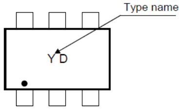
Fig. 9.4 Marking RN2904FE
