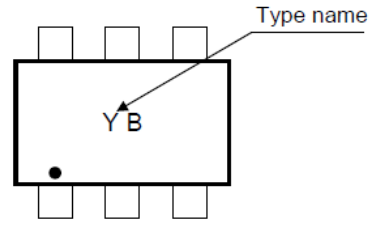
Fig. 9.2 Marking RN2902FE
