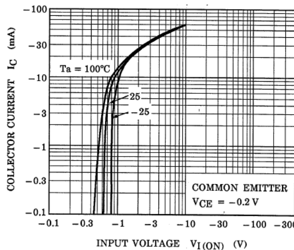
Fig. 10.5 RN2905FE I_C - V_{I(ON)}
