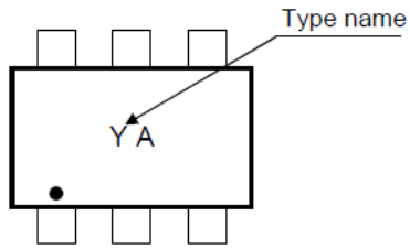
Fig. 9.1 Marking RN2901FE
