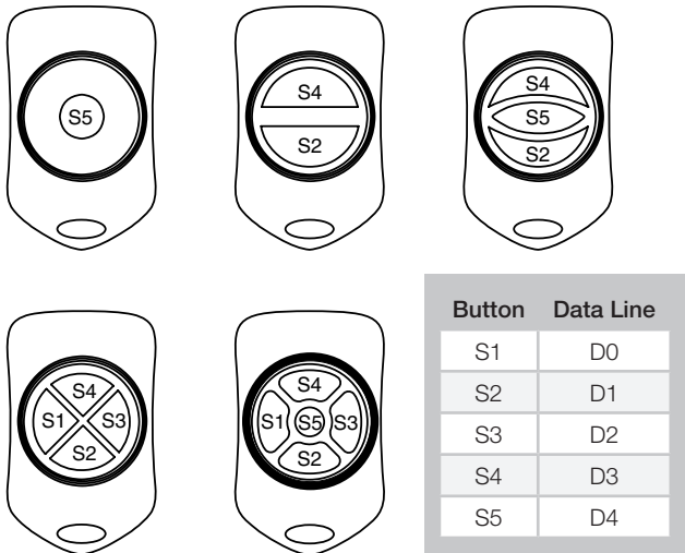
Figure 6: OTX-***-HH-KF#-DS Button Assignments
